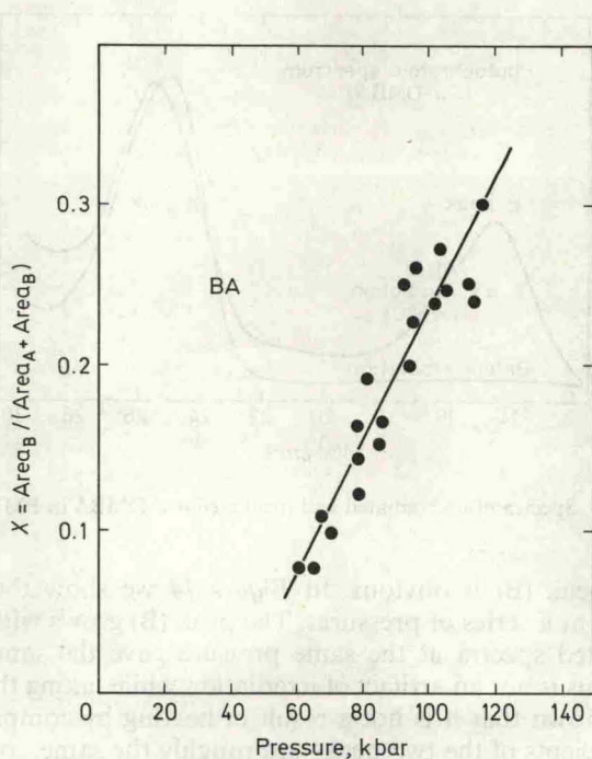
Figure 15. Conversion from A to B form against pressure: BA in PMMA
