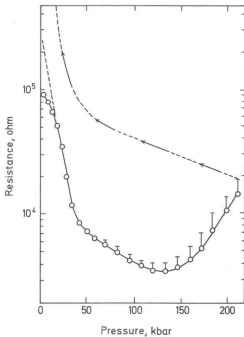
Figure 7. Resistance against pressure: pyrene · 2I 2 complex
