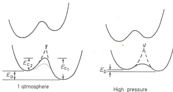
Figure 16. Configuration coordinate diagram for conversion between A and B forms
